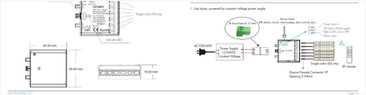
WIRING DIAGRAM
